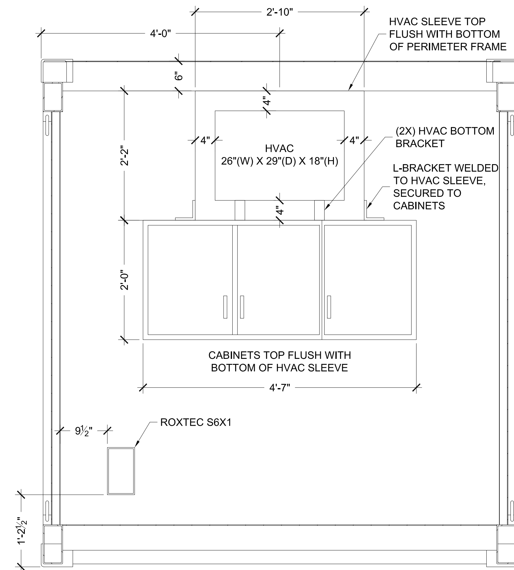
A HVAC WALL INTERIOR ELEVATION A1.1 NTS
